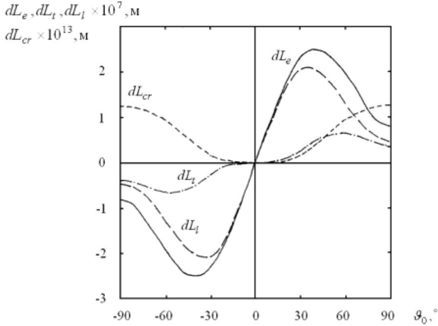
Fig. 1. The dependences of the equivalent path difference dL_e , the longitudinal component of path difference dL_t , the transverse component of path difference dL_l with light dragging effect for two EM waves, one of which propagated in a medium with \omega = 0 , and another with \omega \neq 0 , on the incident angle \mathcal{G}_0 onto a boundary of two media with account of shift of an EM radiation exit point on a surface of an optical disk. The dependence of the equivalent path difference due to bend of a trajectory without shift of an EM radiation exit point is presented as dL_{cr}(\mathcal{G}_0) .
